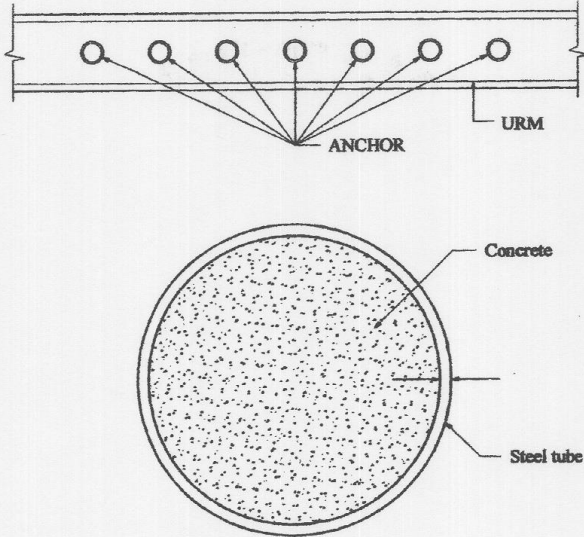
FIGURE 1—CINTEC ANCHOR
