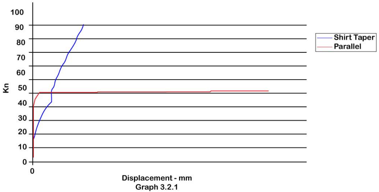
T1- Example of Taper and Parallel Pull Out Loads. Cintec Anchor, 20 mm Grip Bar, 450 mm long. Rapid Grout. 06/06/02
