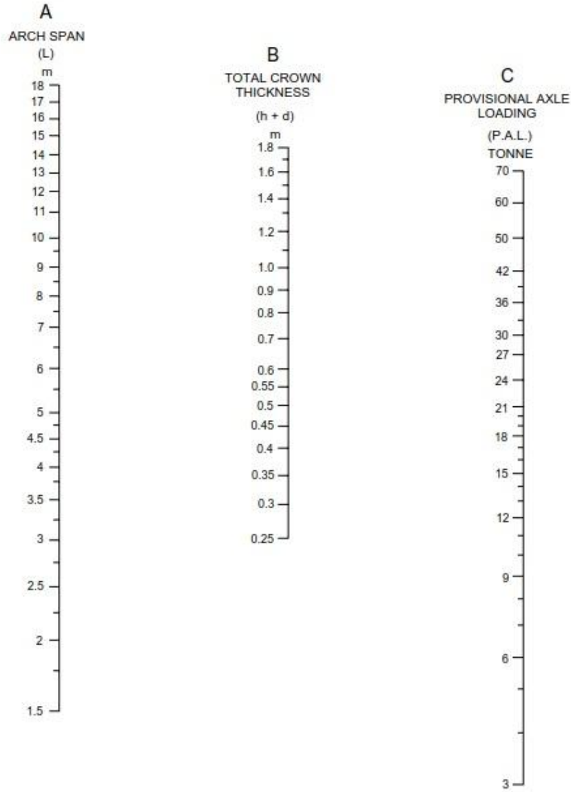
Figure E.1 Nomogram for determining the provisional axle loading for masonry arch bridges before factoring
