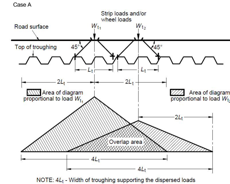
Figure 6.16.1 Dispersal and distribution of load through troughing
