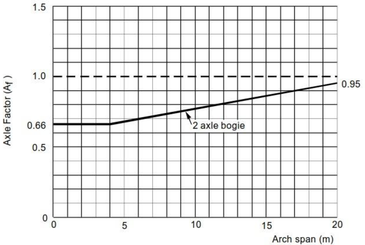
Figure E.6 Axle factor for axle lift-off
