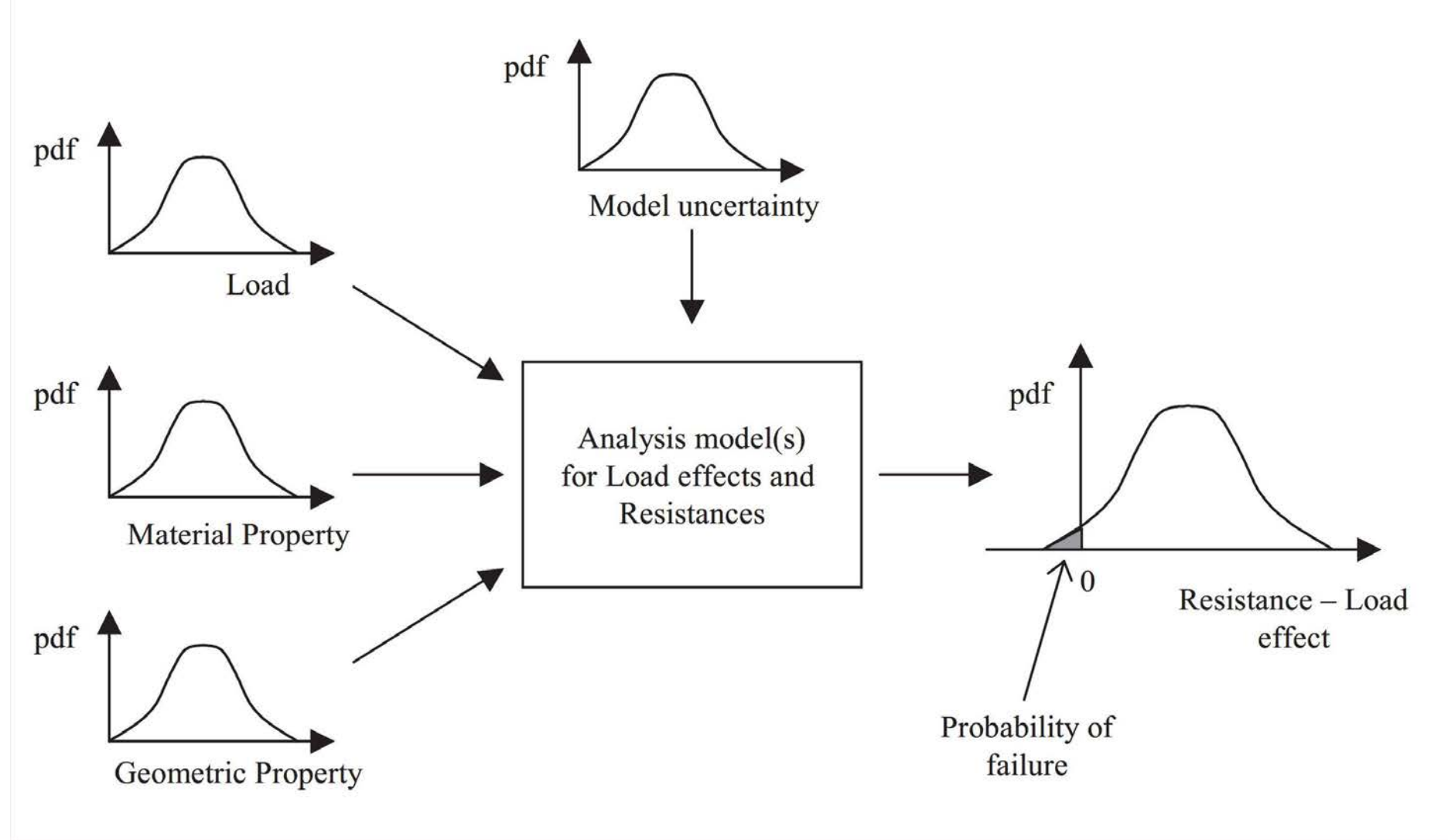
Figure F.2 Illustration of reliability-based methods of assessment
