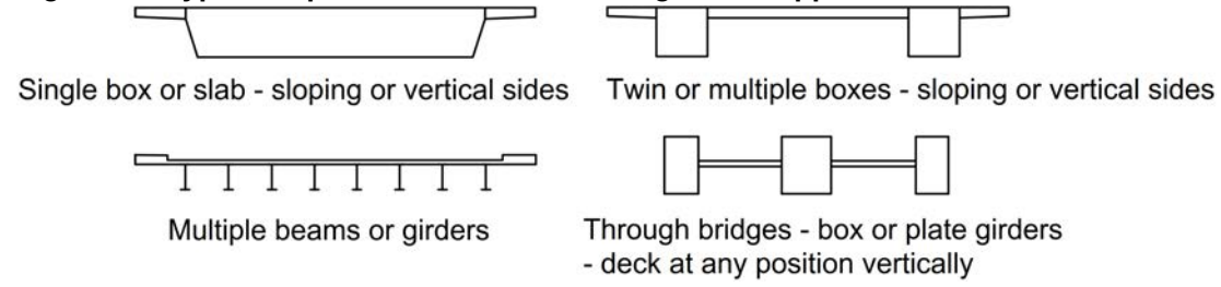
Figure D.5 Typical superstructures to which Figure D.6 applies
