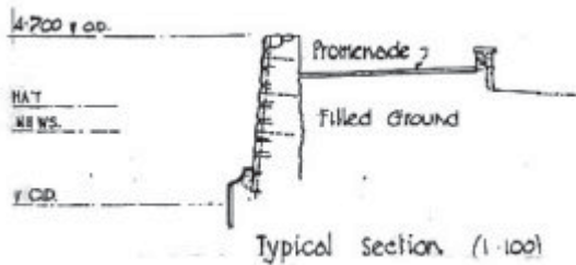
Goodington Sea Wall - Sliding & Delamination
