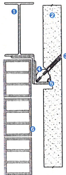
Wall section detail
