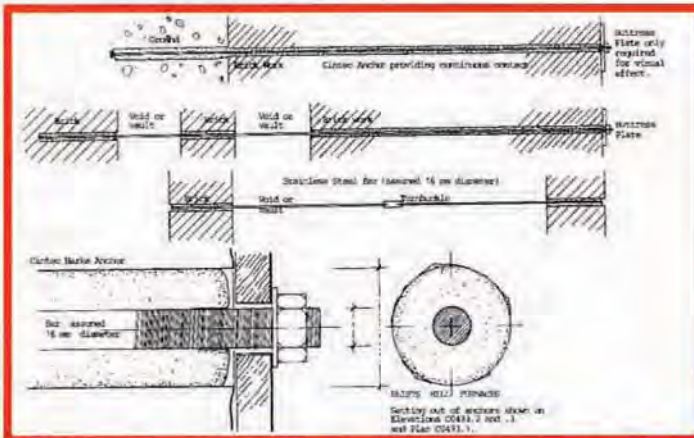
Application of tie bar system with Cintec Anchors covering the south and north furnaces and north engine house.
