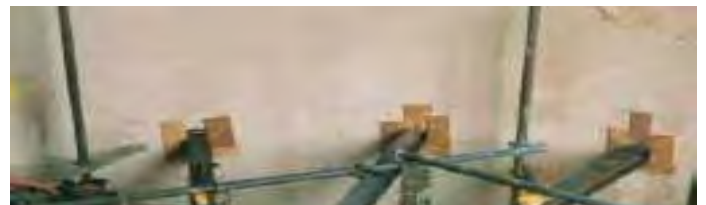
All installed `I` beams leveled and supported as grout Hardens
