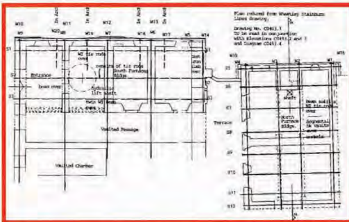
Setting out anchor/tie bars
