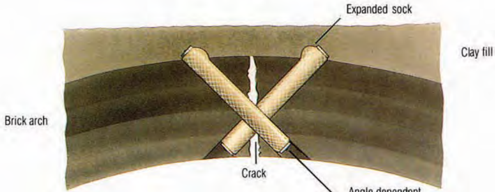
Typical Brick Stitching Anchor Detail to brick Arch
