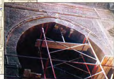
One of the four arches of the court being scaffolded prior to drilling and anchoring
