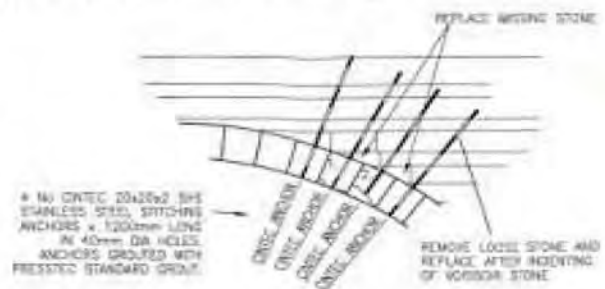
PART ELEVATION OF VOUSSOIRS/SPANDEL FACE
