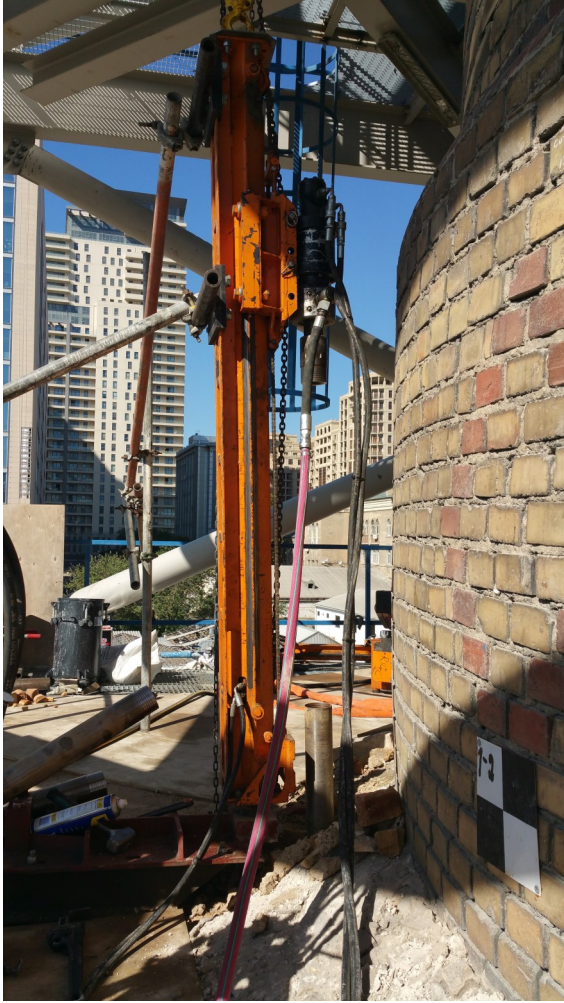
Lower 15mt long Grip Bar 33mm anchors installed in the Octagon base finishing in the brickwork foundation below ground level.
